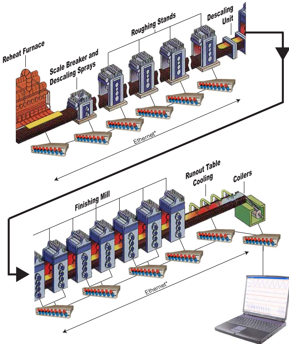
Figure 1. Multiple DI-720 and/or DI-730 products may be connected as a distributed network that covers large distances (each station can be more than 100M apart). All measurements made in such a configuration are synchronized to allow meaningful troubleshooting and fault correction.
