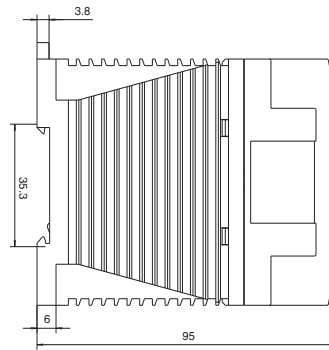
Side View (dimensions in mm)
